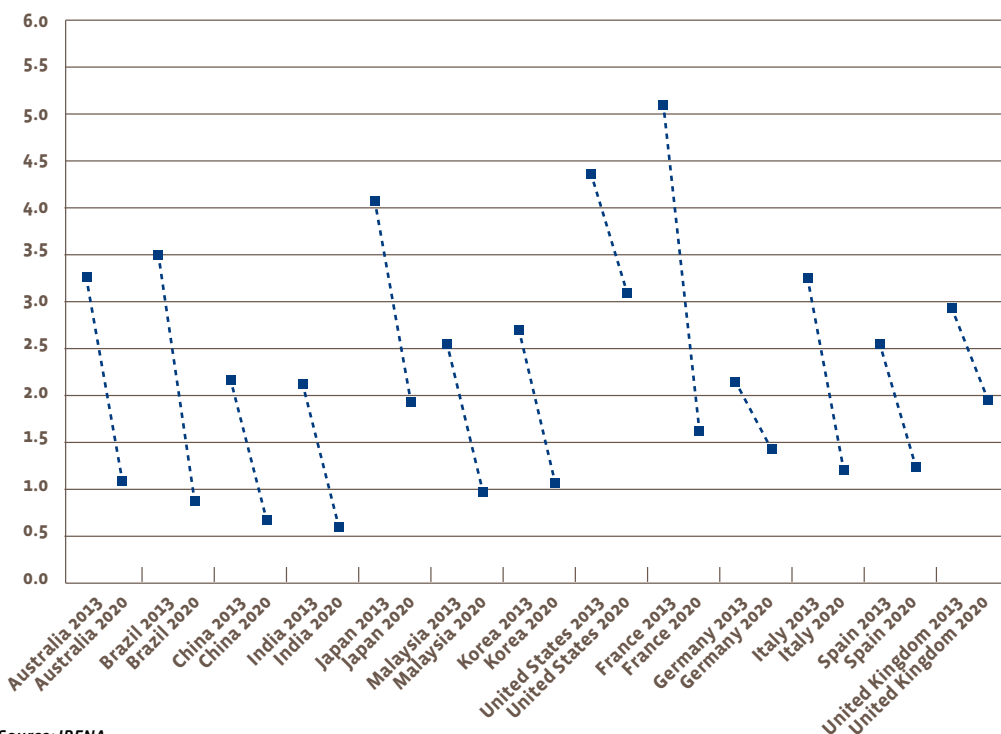
Residential Solar PV investment costs according to IRENA (M€/MWP)
